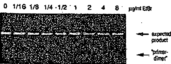
FIGURE 2 Gel electrophoresis of PCR amplification products of the human nuclear gene, HLA DQA1, made in the presence of increasing amounts of EtBr (up to 8 µg/ml). The presence of EtBr has no obvious effect on the yield or specificity of amplification.
